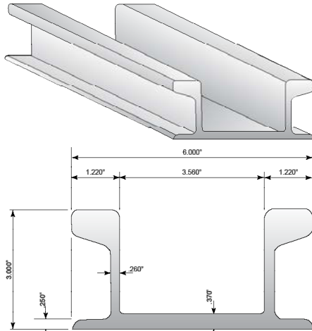
Cross Section of Standard Waler
