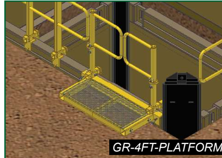
Guard Rail Platform with Closed Gate
