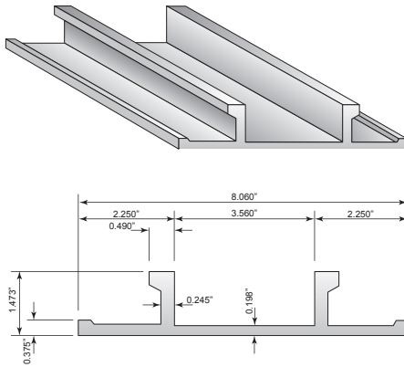
Cross Section of Standard Vertical Rail
