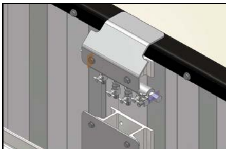
Close Up - Manifold on Shield
