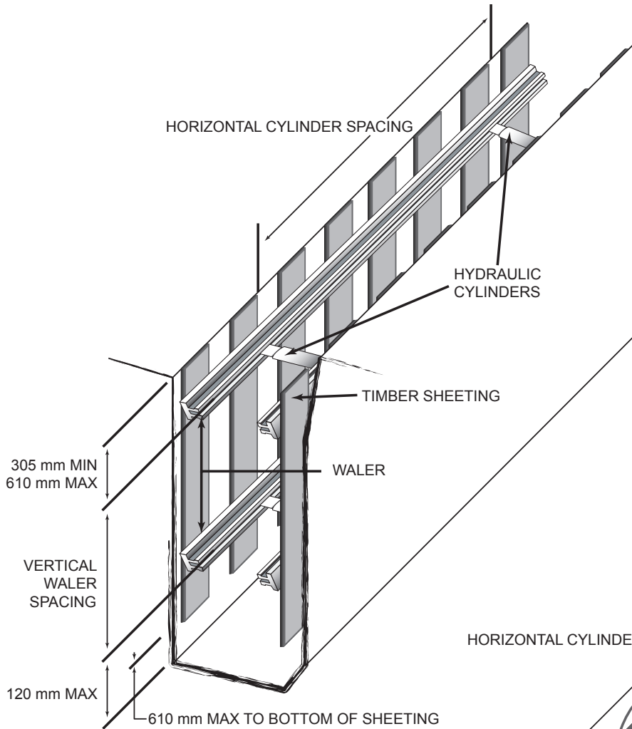
Soil Type A & B with timber
