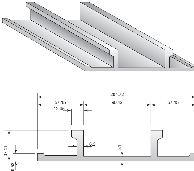
Cross Section of Standard Vertical Rail Dimensions Millimeter (mm)
