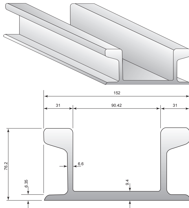
Cross Section of Standard Waler Dimensions Millimeter (mm)
