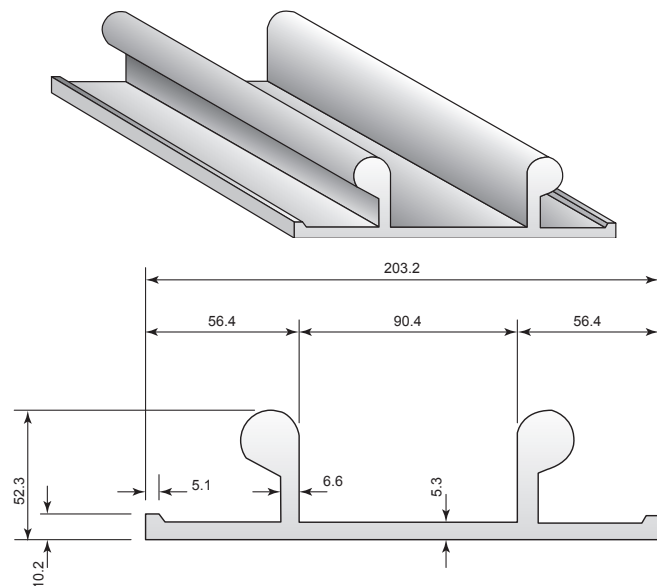
Cross Section of Heavy-Duty Vertical Rail Dimensions Millimeter (mm)
