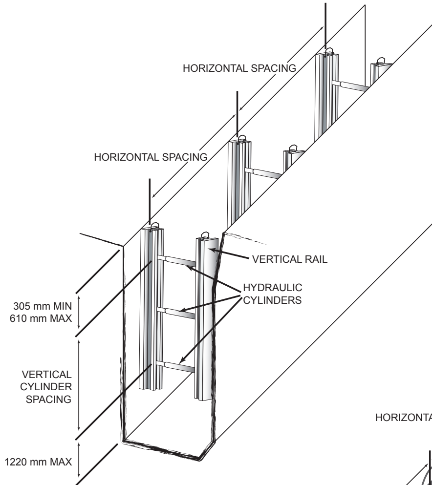
Soil Type A & B without plywood
