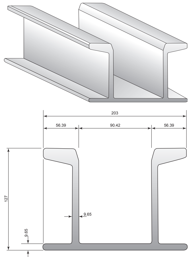
Cross Section of Heavy-Duty Waler Dimensions Millimeter (mm)
