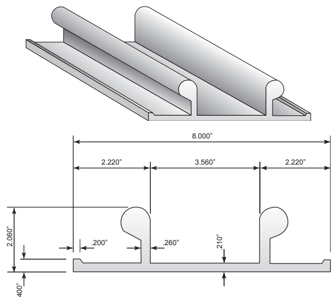
Cross Section of Heavy-Duty Vertical Rail
