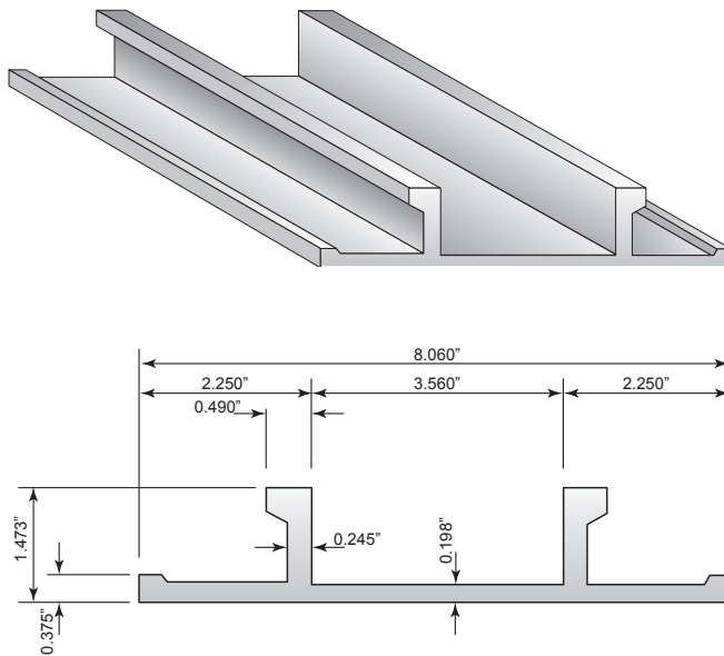
Cross Section of Standard Vertical Rail
